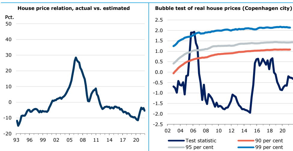
Empirical models
