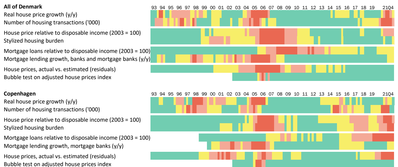
Heat map
